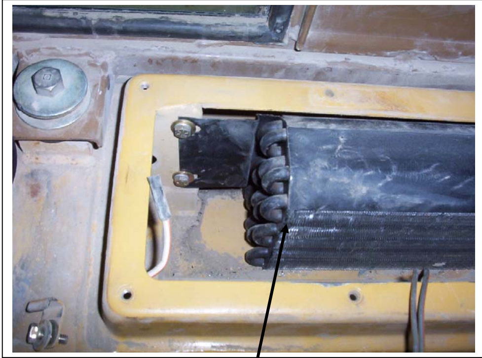
Evaporator location
